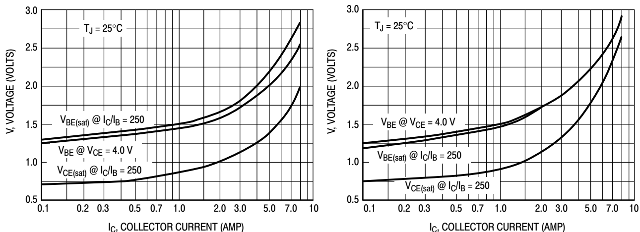
Figure 10. "On" Voltages
