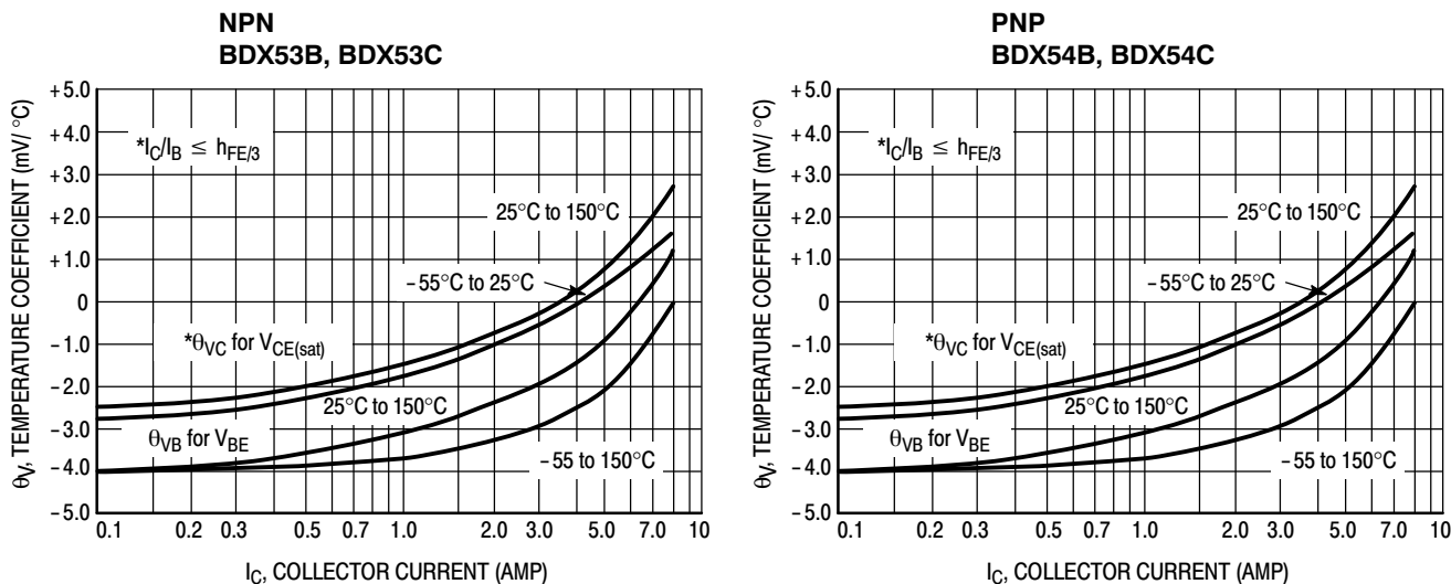
Figure 11. Temperature Coefficients
